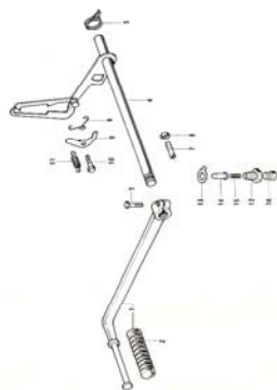
9. Gear Change Mechanism
