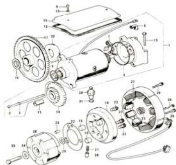
16. Starter Motor, Dynamo
