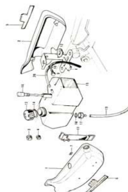
29. Oil Tank, Side Covers
