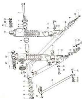
18. Swinging Arm, Rear Shock Abs.
