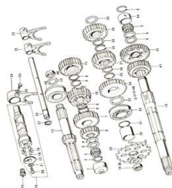
8. Transmission Gears 2/2
