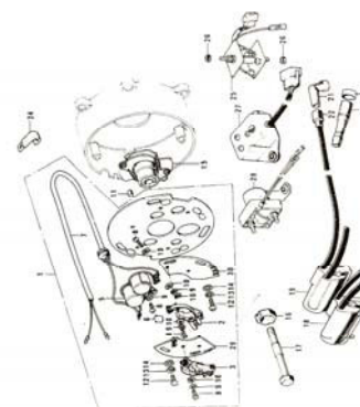
15. Contact Breaker
