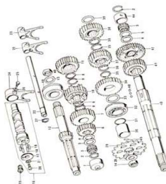
8. Transmission Gears 1/2
