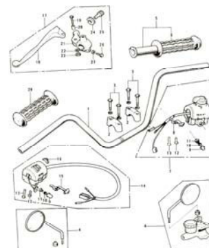
20. Handlebar, Grips
