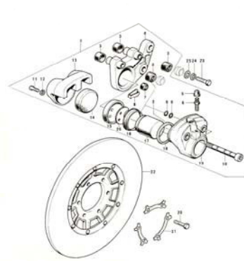
26. Disc Brake Equipments B
