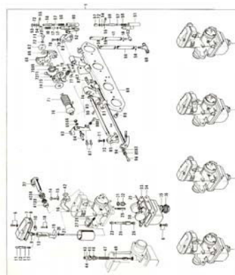
12. Carburetors 3/3
