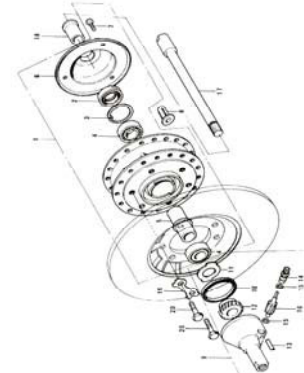
23. Front Hub
