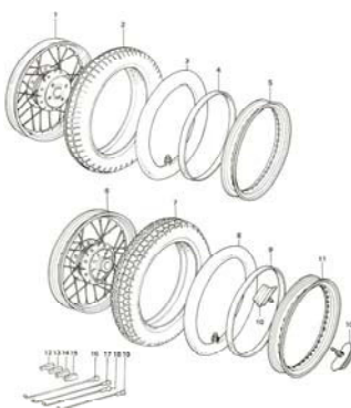
22. Wheels
