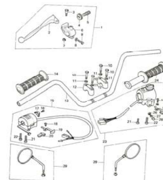
20. Handlebar, Grips
