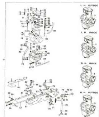
12. Carburetors 3/3
