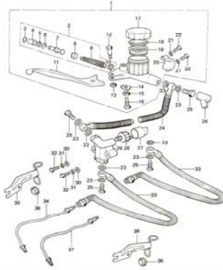
25. Disc Brake Equipments A
