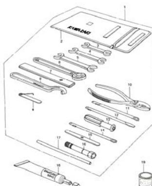
36. Tools
