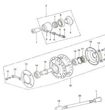
23. Front Hub
