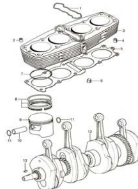
3. Cylinder, Piston, Crank Shaft
