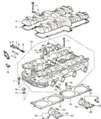
1. Cylinder Head
