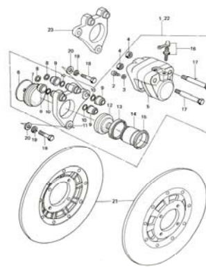
26. Disc Brake Equipments B
