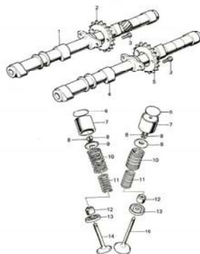
2. Cam Shaft, Valve
