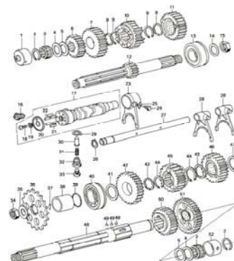
8. Transmission Gears 2/2
