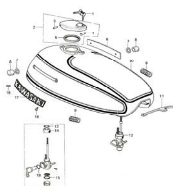
28. Fuel Tank
