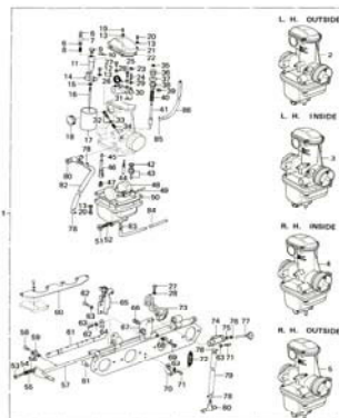
12. Carburetors 2/3
