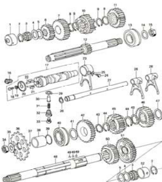
8. Transmission Gears 1/2
