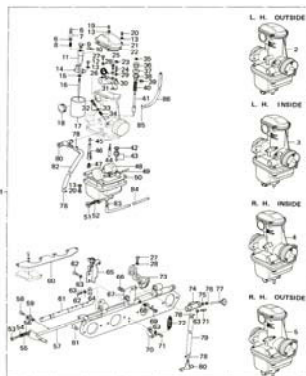
12. Carburetors 1/3
